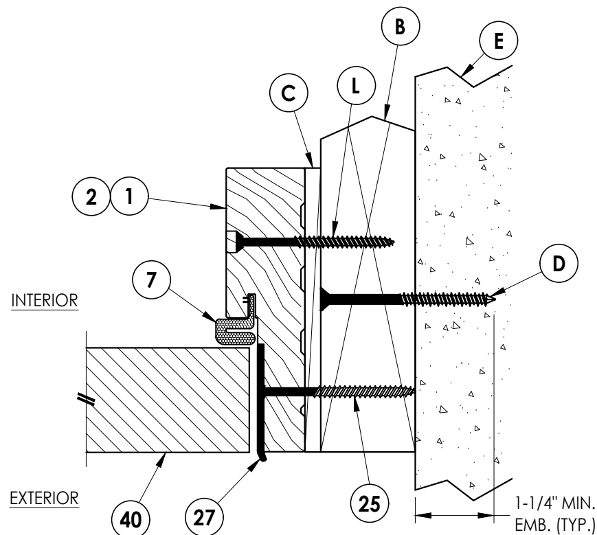
3 7 HORIZONTAL CROSS SECTION Outswing Shown (Inswing Similar) Shown w/ 2X Buck
