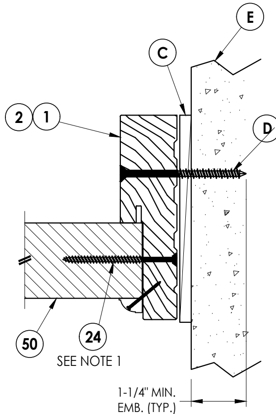
2 9 HORIZONTAL CROSS SECTION Outswing Shown (Inswing Similar) Shown Direct to Masonry
