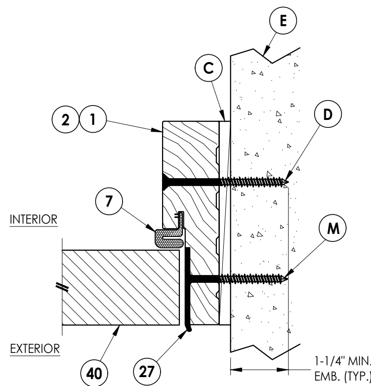
3 9 HORIZONTAL CROSS SECTION Outswing Shown (Inswing Similar) Shown Direct to Masonry
