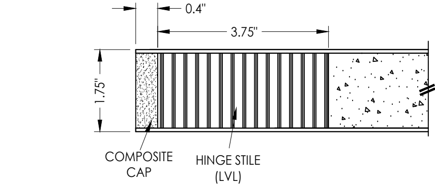
1 2 HORIZONTAL CROSS SECTION
